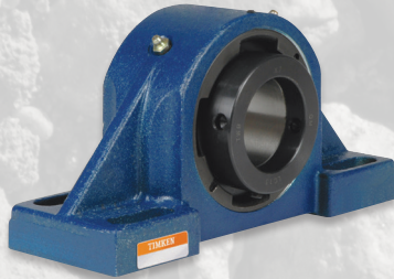
SOLID-BLOCK MOUNTED SPHERICAL ROLLER BEARINGS Heavy-duty Protection, High Performance
