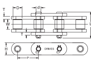
Straight style small roller
