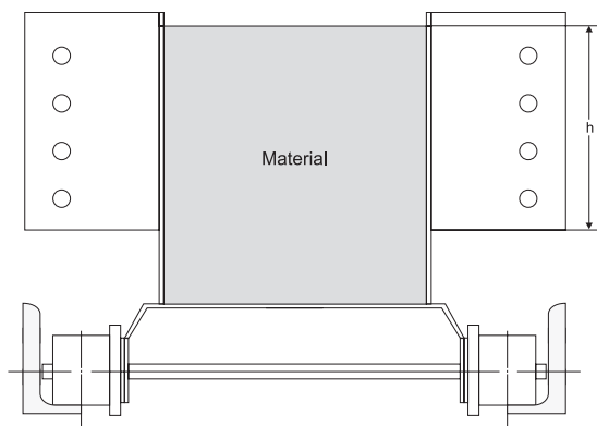
Fig. 6. Cross-section of material conveyed in a trough.
