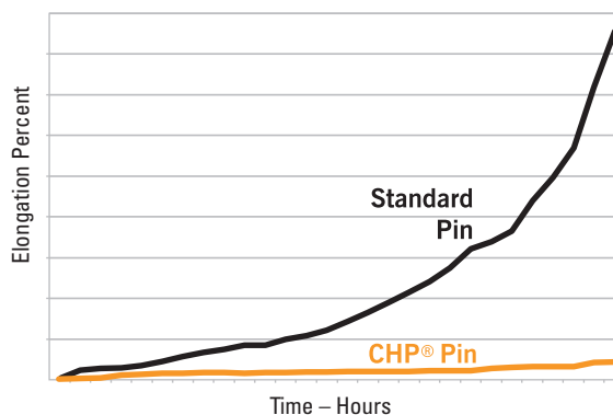
Fig. 35. Elongation vs. time.
