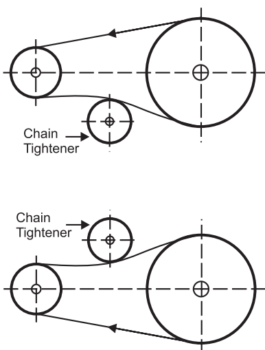
Fig. 13. When the slack side is on top, some means must be provided to adjust the slack-side tension.
