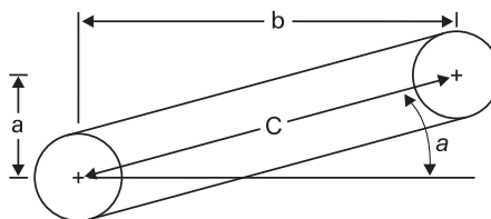
Fig. 5. Inclined - return side supported illustration.
