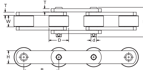
Straight style large roller
