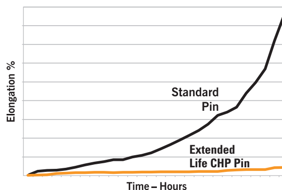
Fig. 38. Elongation vs. time.
