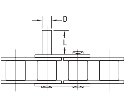
Single pin
