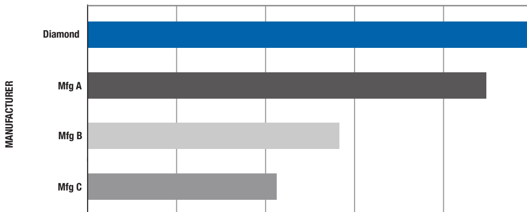
ISO/British Standard 10B-1 Accelerated Wear Test (time to wear limit)
